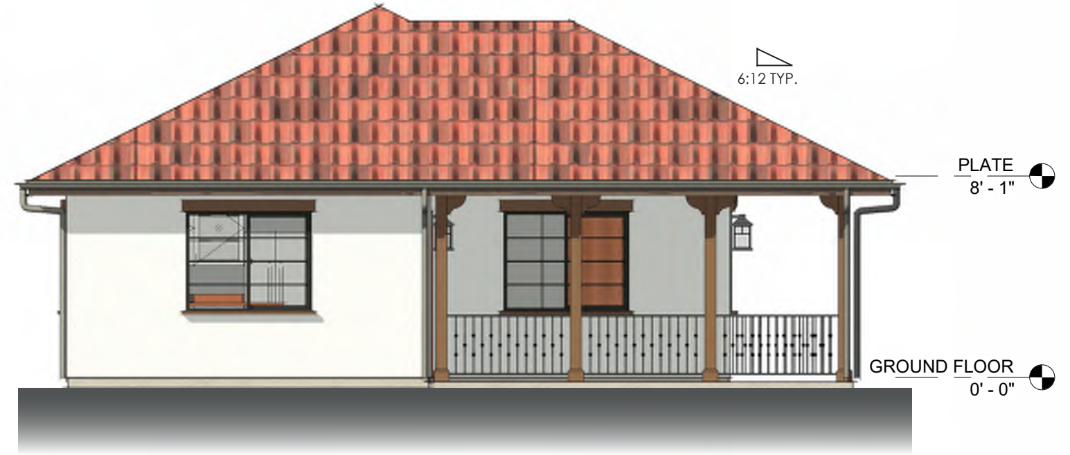
2 LEFT ELEVATION 3/16" = 1'-0" (12 X 18 SHEET)
