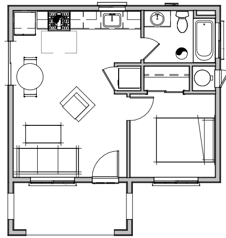
① PLAN 1 | STYLE A | 480 FT 2 3/32" = 1'-0" (12 X 18 SHEET)
